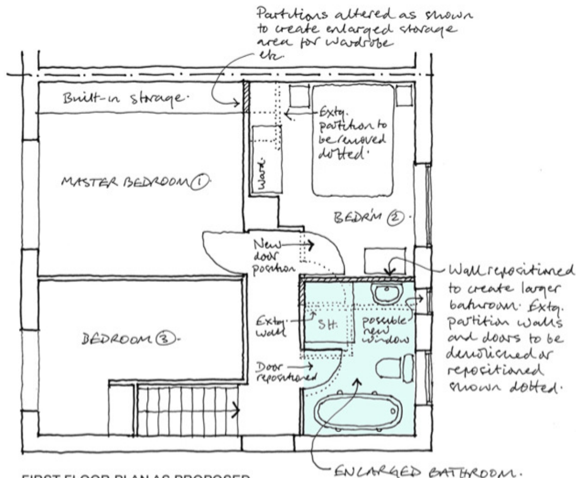
FIRST FLOOR PLAN AS PROPOSED
