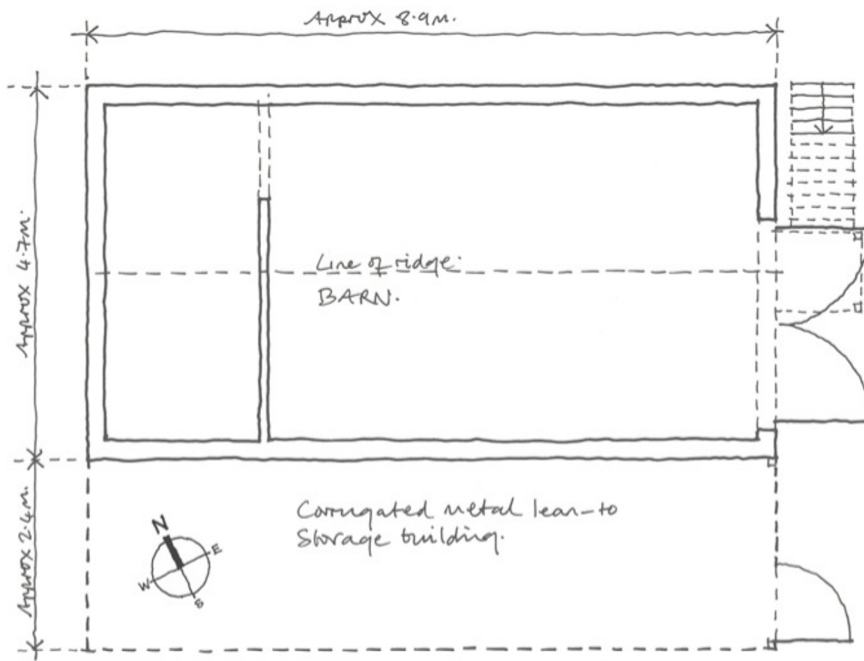
BARN PLAN AS EXISTING
