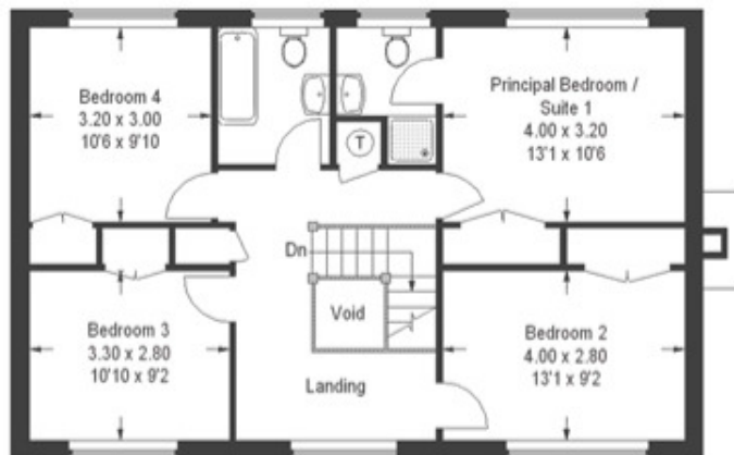
FIRST FLOOR PLAN AS EXISTING
